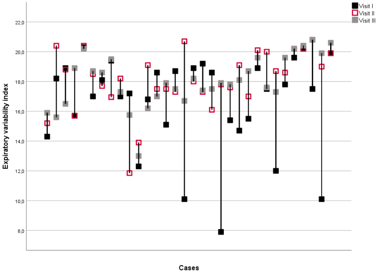
FIGURE 1. Expiratory variability index at every visits for 32 children. In total 19 of 32 children lowest value were observed at Visit I before starting inhaled corticosteroid.
